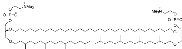
Figure 1. Structure of archae phospholipid, L-32-Phy.
