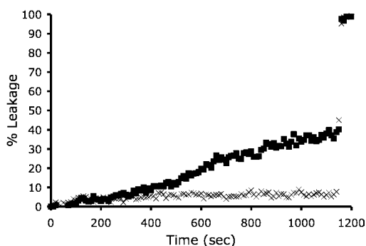
Figure 3. Leakage induced upon addition of bolaamphiphile to vesicles containing carboxyfluorescein (50 mM). To 25 \mu M of 8:2 POPC/cholesterol vesicles in TES buffer (5 mM TES, 100 mM NaCl, pH 7.4) was added 10 \mu M of para-isomer 6 (■) or meta-isomer 7 (×) at 50 s, and the vesicles were lysed by addition of Triton X-100 at 1150 s. Repeating the experiment with amphiphiles 4 , 5 , and 8 yielded the same result as 7 , that is, no leakage.
